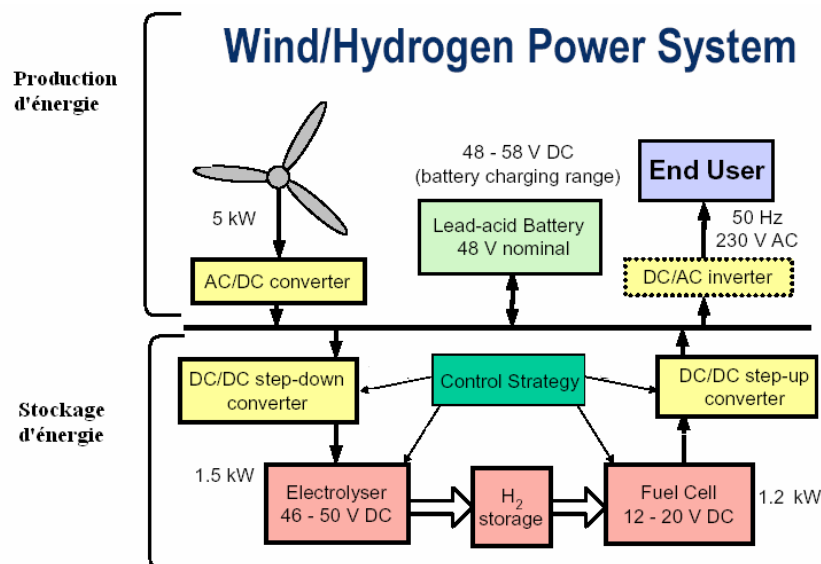
Figure 2: Example of a Wind hydrogen fuel cell test bench configuration (NATO SfP-982620)
