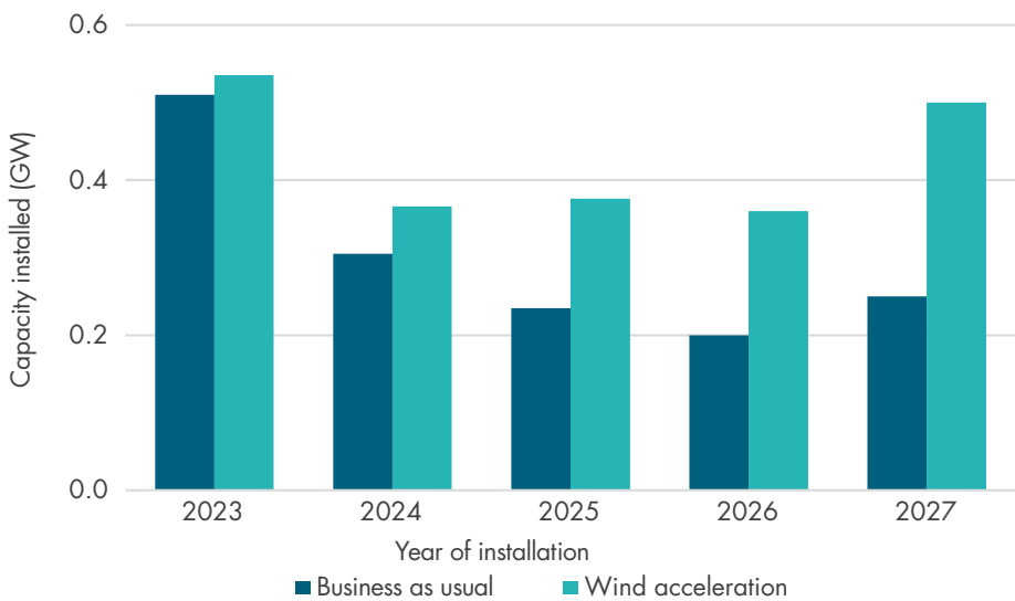
Figure 27 Forecast of installed capacity in Morocco in the two scenarios.
