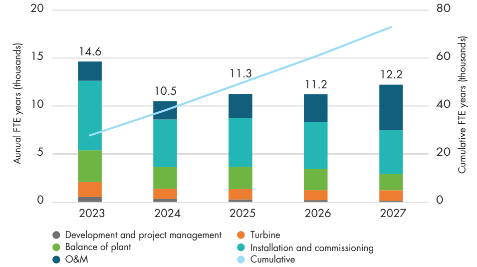
Figure 29 FTE years created in the wind acceleration scenario in Morocco.
